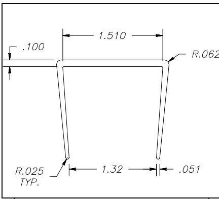
D*80892 1.5" C-Channel
