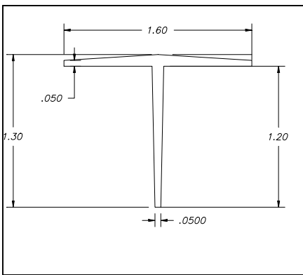
D*80751 T-Strip
