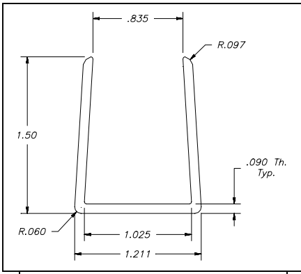
F*39108 1" C-Channel
