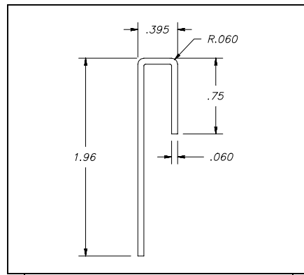
D*42603 J-Channel
